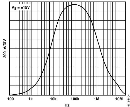
Figure 41. Band-Pass Response
