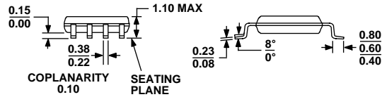
Figure 44. 8-Lead Mini Small Outline Package [MSOP] (RM-8)
