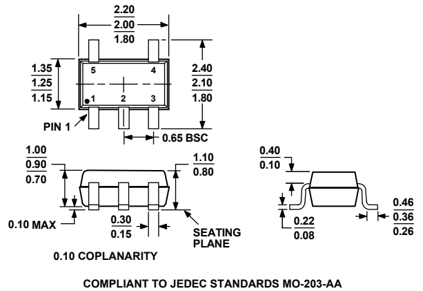
COMPLIANT TO JEDEC STANDARDS MO-203-AA Figure 36. 5-Lead Thin Shrink Small Outline Package [SC70] (KS-5) Dimensions shown in millimeters
