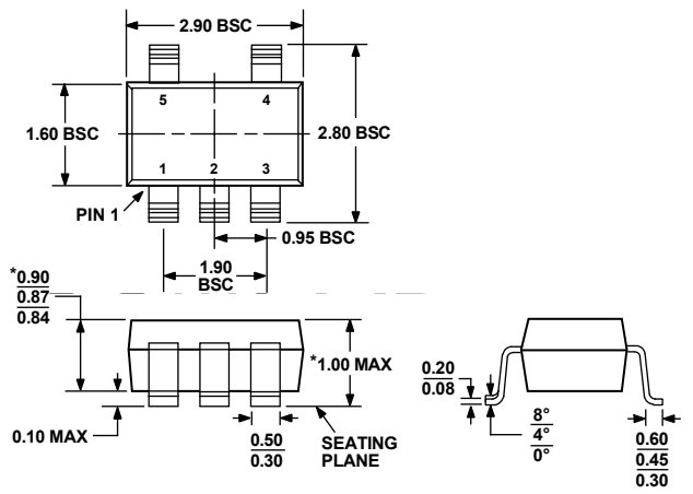
*COMPLIANT TO JEDEC STANDARDS MO-193-AB WITH THE EXCEPTION OF PACKAGE HEIGHT AND THICKNESS. Figure 37. 5-Lead Thin Small Outline Transistor Package [TSOT] (UJ-5) Dimensions shown in millimeters
