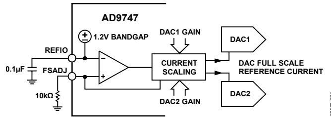
Figure 33. Reference Circuitry
