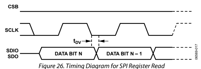
Figure 26. Timing Diagram for SPI Register Read
