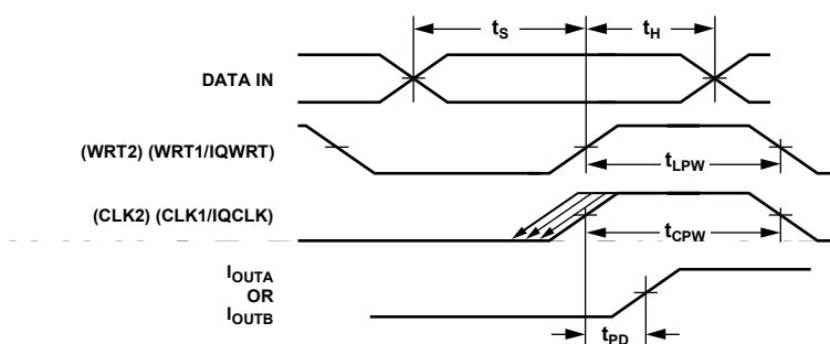
Figure 2. Timing Diagram for Dual and Interleaved Modes
