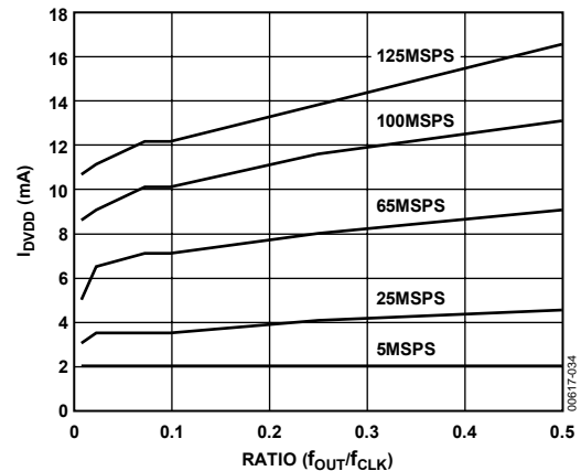
Figure 34. I_{DVDD} vs. Ratio @ DVDD = 3.3 V
