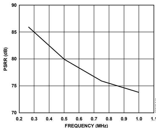
Figure 40. Power Supply Rejection Ratio
