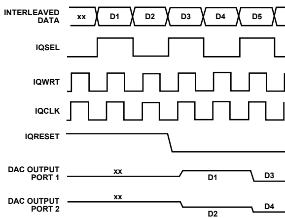
Figure 29. Interleaved Mode Timing
