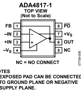
Figure 6. ADA4817-1 Pin Configuration (8-Lead SOIC)
