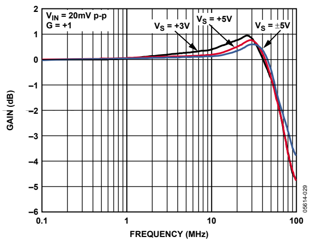
Figure 10. Small Signal Frequency Response vs. Supply Voltage
