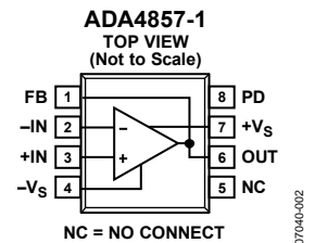
Figure 2. 8-Lead SOIC (R)
