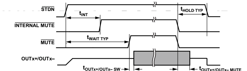
Figure 3. Timing Diagram (Typical)
