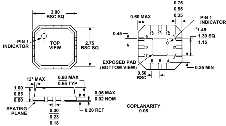
*COMPLIANT TO JEDEC STANDARDS MO-220-VEED-1 EXCEPT FOR EXPOSED PAD DIMENSION. Figure 27. 12-Lead Lead Frame Chip Scale Package [LFCSP_VQ] 3 mm × 3 mm Body, Very Thin Quad (CP-12-1) Dimensions shown in millimeters
