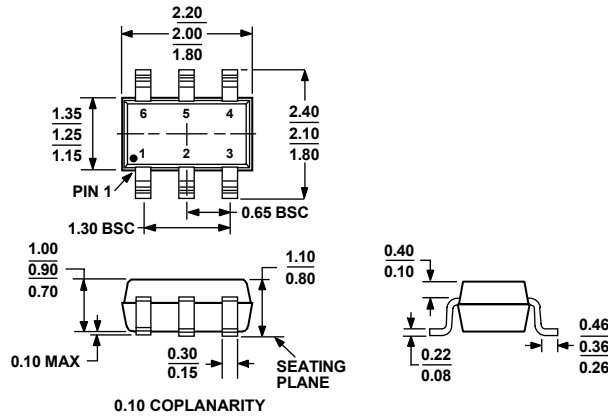
COMPLIANT TO JEDEC STANDARDS MO-203-AB Figure 26. 6-Lead Thin Shrink Small Outline Transistor Package [SC70] (KS-6) Dimensions shown in millimeters
