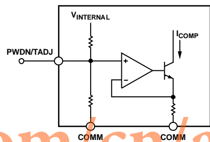
Figure 35. TADJ Interface
