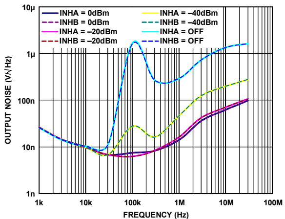
Figure 42. Noise Spectral Density of OUTA, OUTB; CLPA, CLPB = Open
