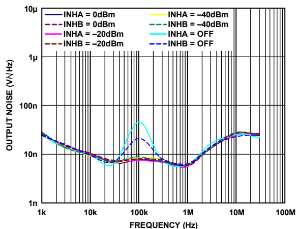
Figure 44. Noise Spectral Density of OUTA, OUTB; CLPA, CLPB = 0.1 μF, Frequency = 2140 MHz
