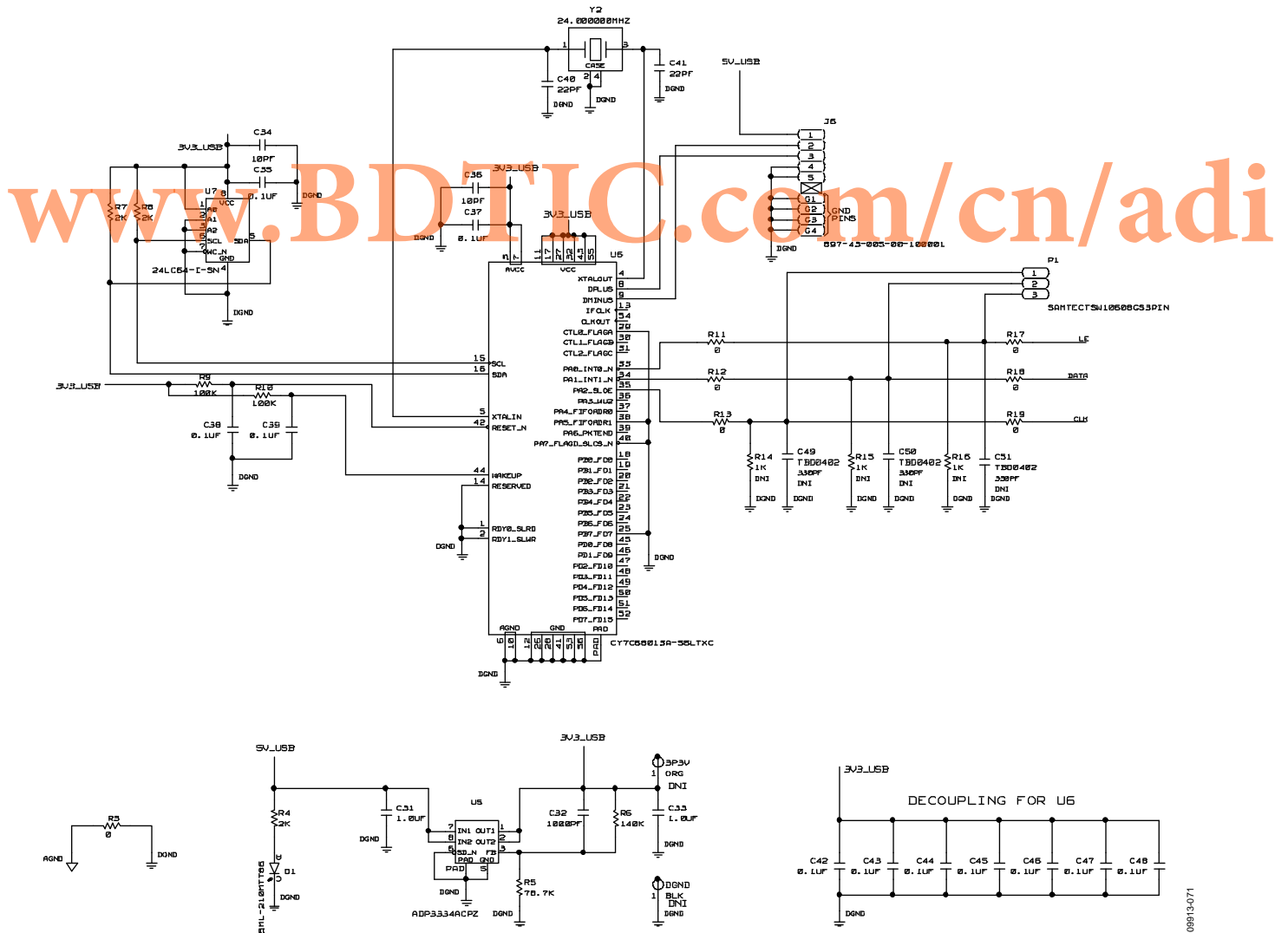
Figure 65. USB Interface Circuitry on the Evaluation Board
