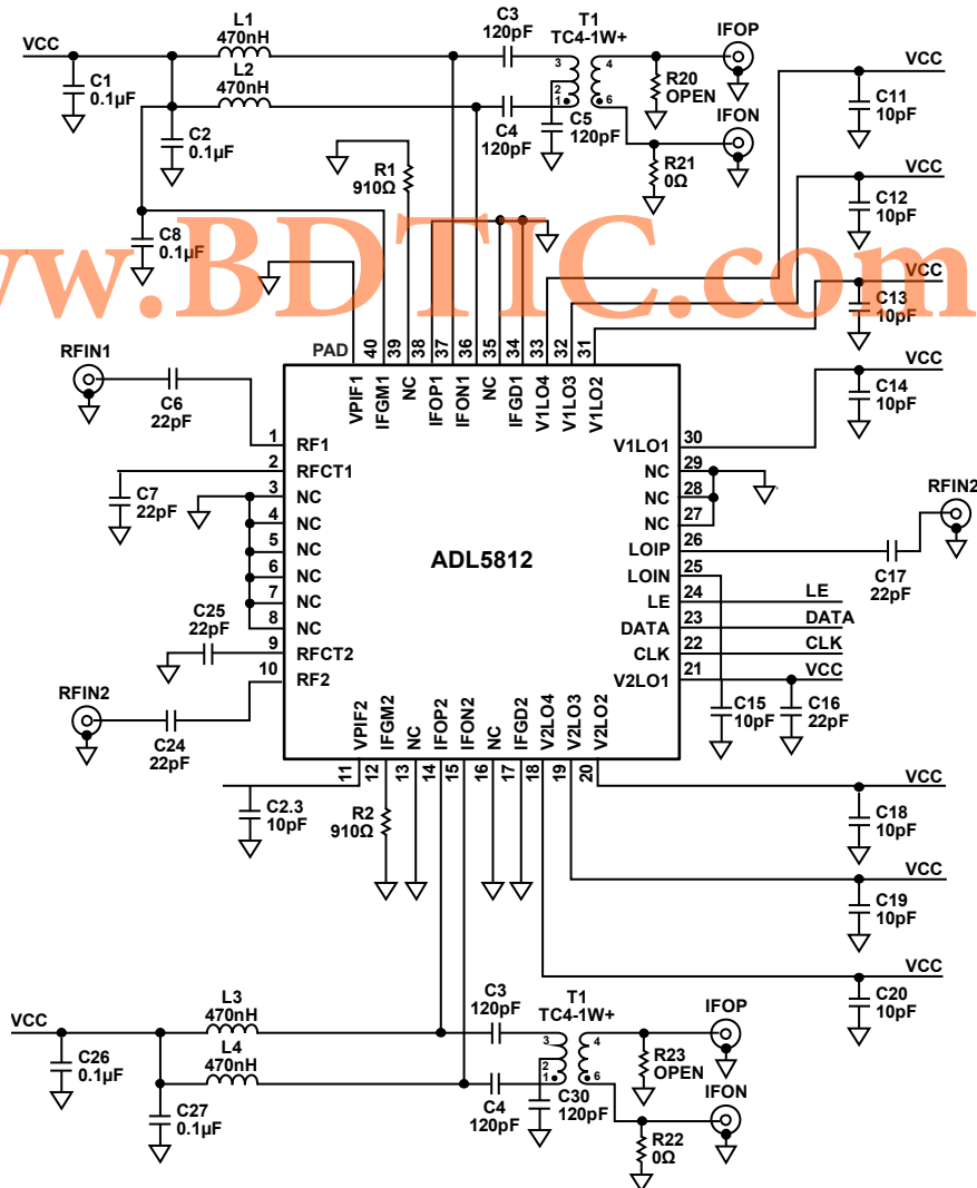
Figure 60. Evaluation Board Schematic
