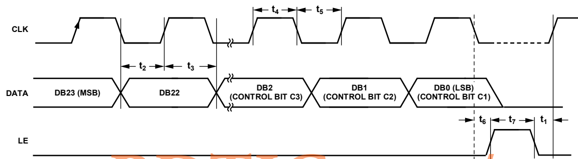
Figure 2. Timing Diagram
