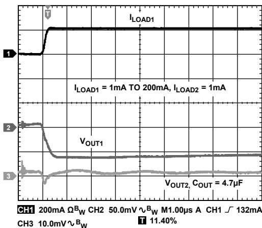
Figure 30. Output Transient Response I_{LOAD1} = 1 \text{ mA TO } 200 \text{ mA} , I_{LOAD2} = 1 \text{ mA} CH1 = I_{LOAD1} , CH2 = V_{OUT1} , CH3 = V_{OUT2} , C_{OUT} = 4.7 \mu\text{F}
