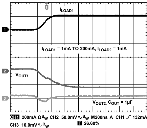
Figure 29. Output Transient Response I_{LOAD1} = 1 \text{ mA TO } 200 \text{ mA} , I_{LOAD2} = 1 \text{ mA} CH1 = I_{LOAD1} , CH2 = V_{OUT1} , CH3 = V_{OUT2} , C_{OUT} = 1 \mu\text{F}
