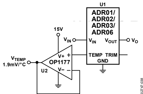
Figure 38. Temperature Monitoring
