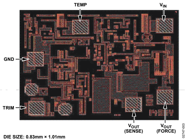
Figure 3. Die Layout
