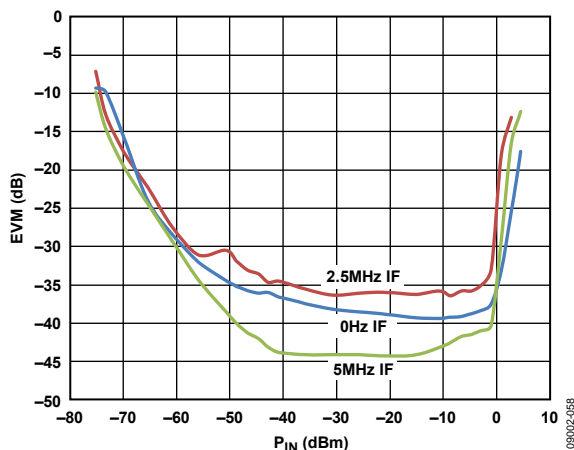
Figure 50. EVM vs. RF Input Power Level; OFDS Pulled Low, C_{OFS} = 1 \mu\text{F}
