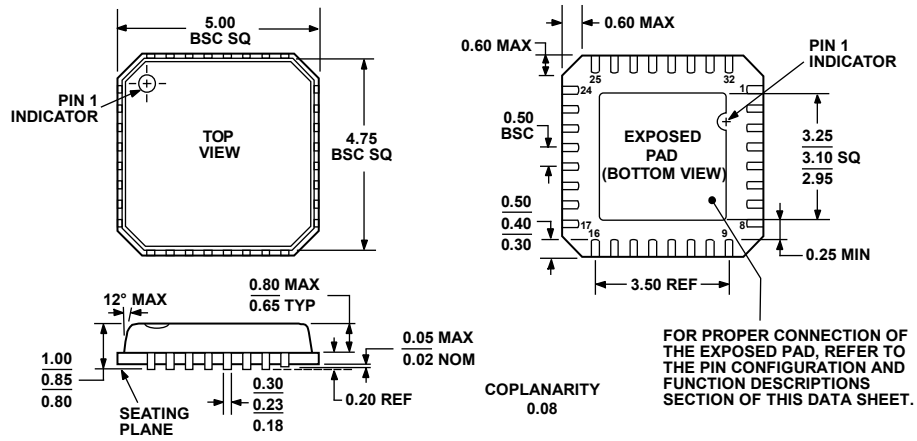
COMPLIANT TO JEDEC STANDARDS MO-220-VHHD-2 Figure 64. 32-Lead Lead Frame Chip Scale Package [LFCSP_VQ] 5 mm × 5 mm Body, Very Thin Quad (CP-32-2) Dimensions shown in millimeters
