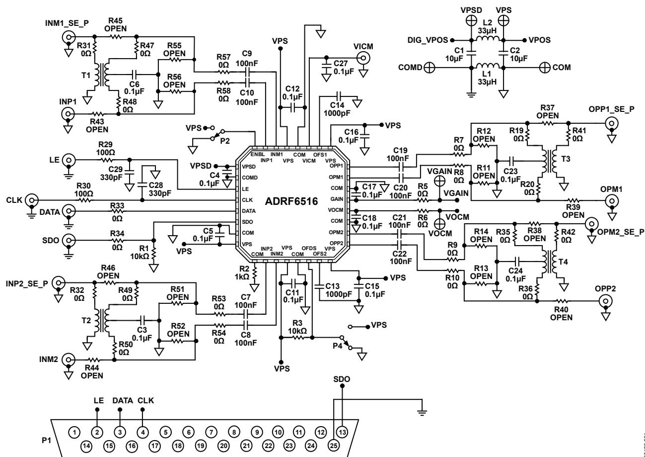
Figure 58. Evaluation Board Schematic
