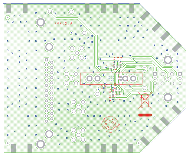
Figure 60. Component Side Layout
