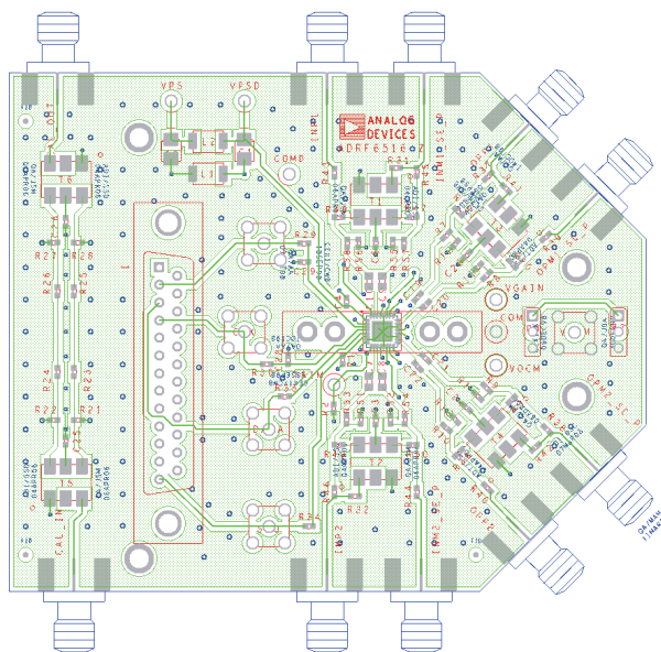
Figure 59. Top Layer Silkscreen
