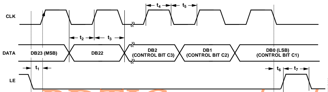
Figure 2. Timing Diagram
