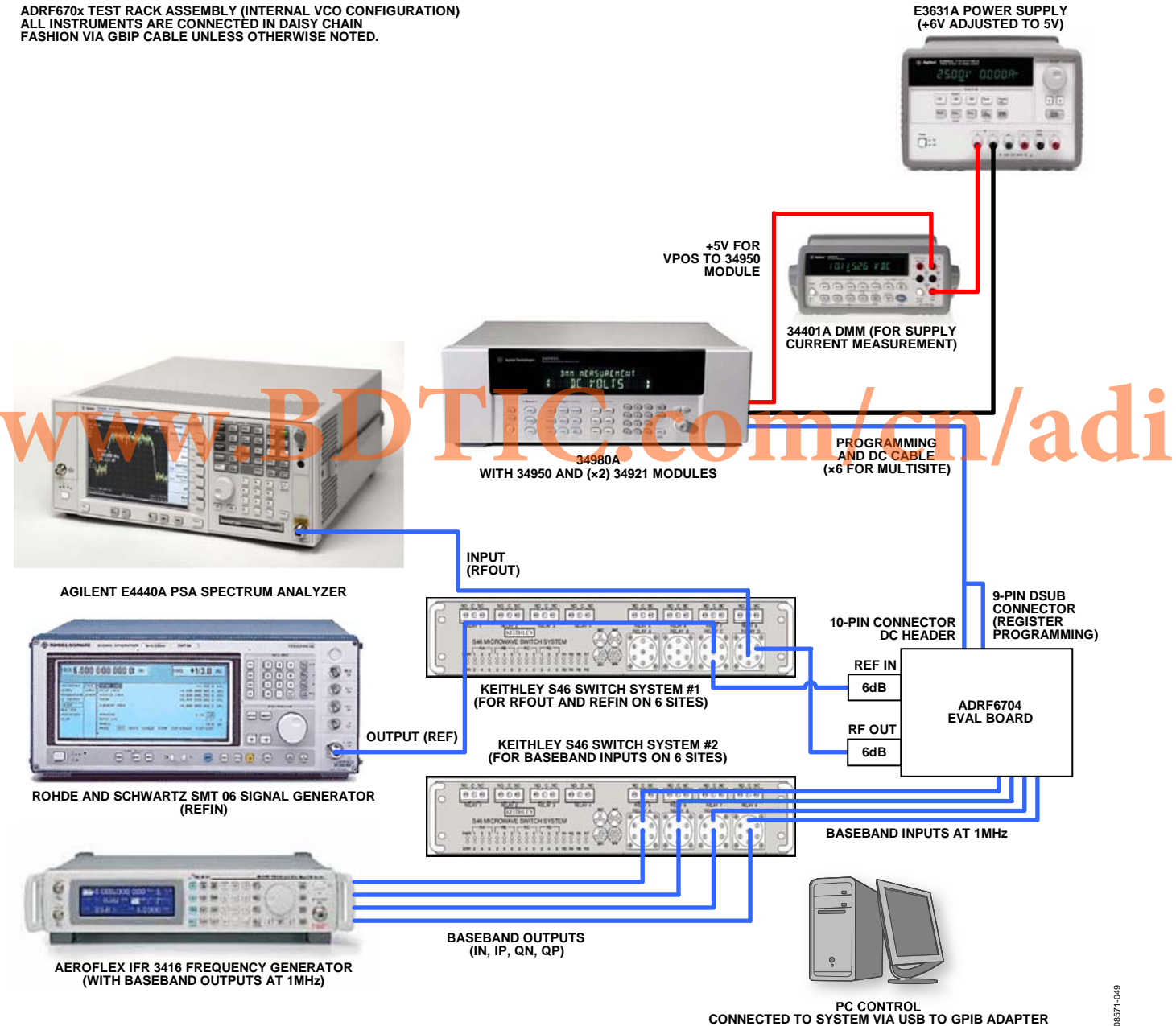
Figure 48. General Characterization Setup
