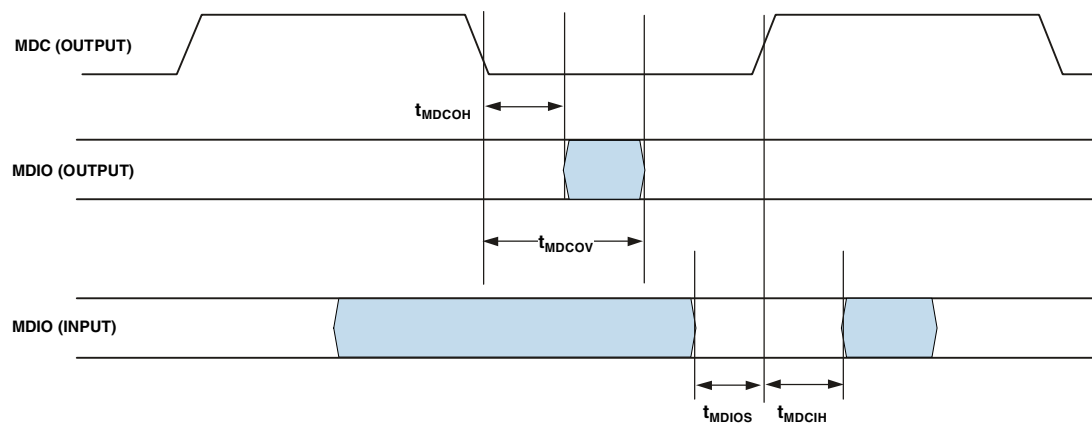
Figure 31. 10/100 Ethernet MAC Controller Timing: MII Station Management
