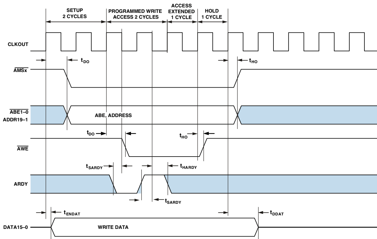
Figure 9. Asynchronous Memory Write Cycle Timing
