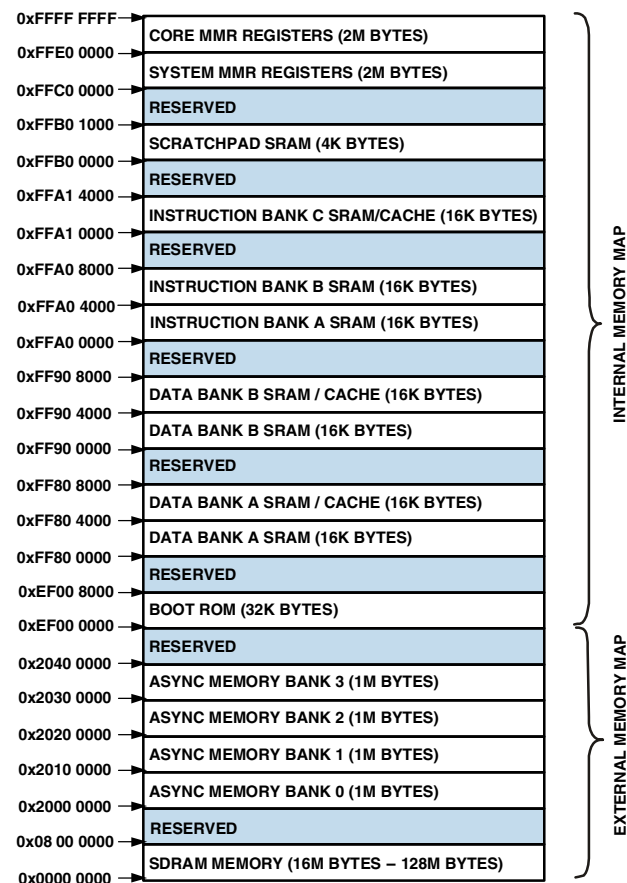
Figure 2. ADSP-BF512/BF514/BF516/BF518(F) Internal/External Memory Map
