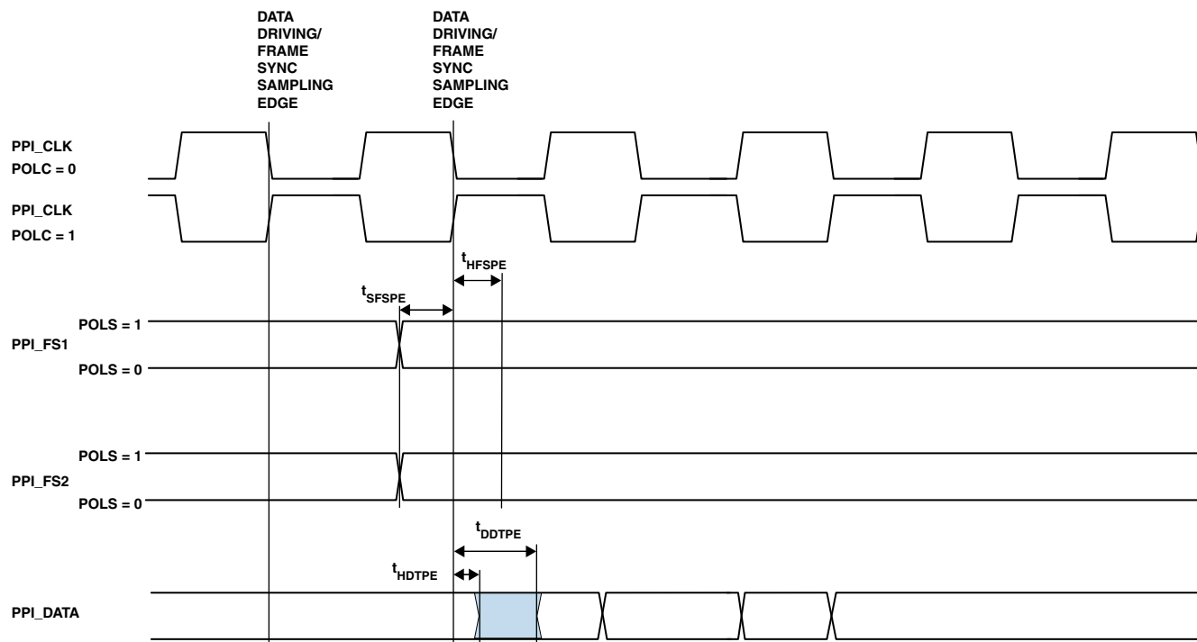
Figure 13. PPI GP Tx Mode with External Frame Sync Timing
