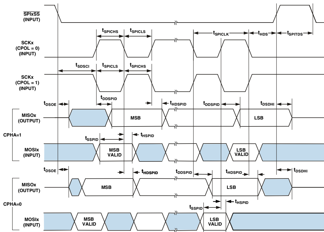
Figure 21. Serial Peripheral Interface (SPI) Port—Slave Timing
