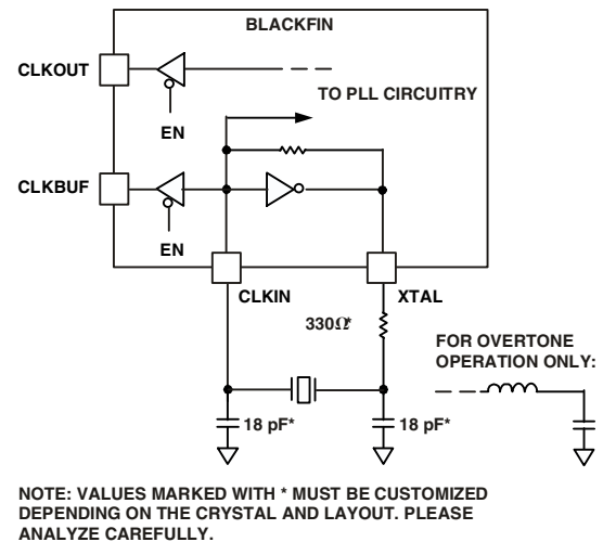
Figure 4. External Crystal Connections
