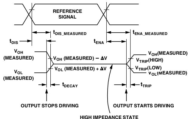
Figure 46. Output Enable/Disable
