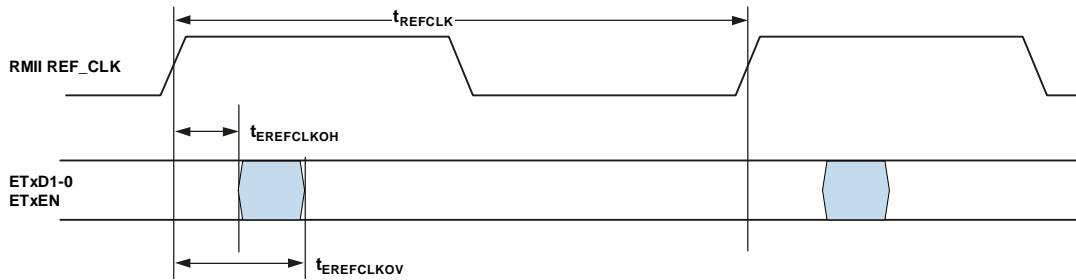
Figure 31. 10/100 Ethernet MAC Controller Timing: RMI Transmit Signal
