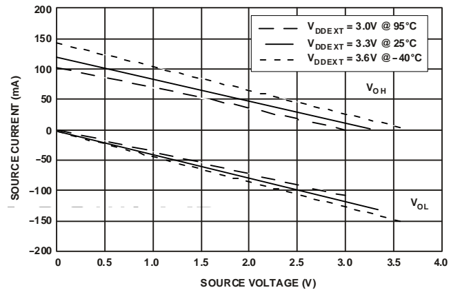
Figure 37. Drive Current B (High V_{DDEXT} )
