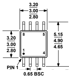
Figure 22. 8-Lead Standard Small Outline Package [SOIC_N] Narrow Body (R-8) Dimensions shown in millimeters and (inches)
