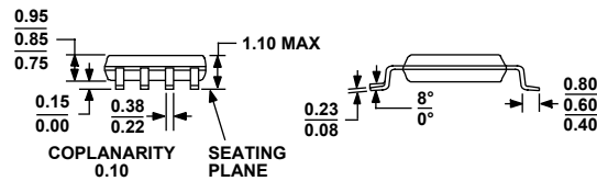
COMPLIANT TO JEDEC STANDARDS MO-187-AA Figure 23. 8-Lead Mini Small Outline Package [MSOP] (RM-8) Dimensions shown in millimeters
