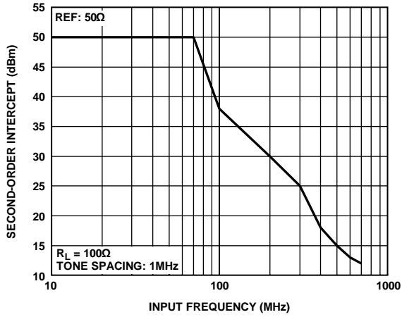
Figure 55. ADV3225 Output Second-Order Intercept, 100 Ω Load
