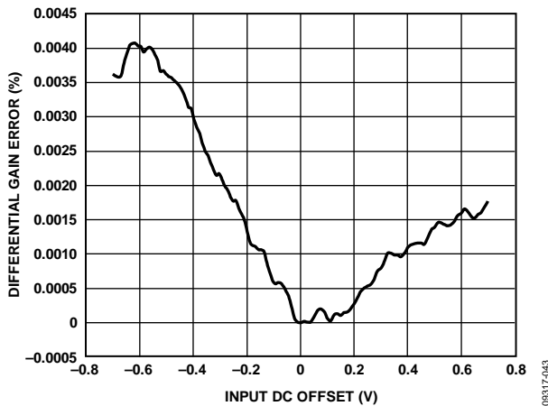
Figure 45. ADV3224 Differential Gain Error
