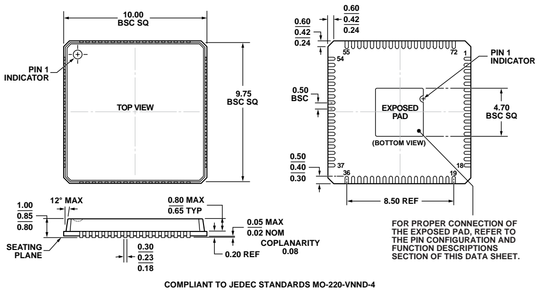
Figure 66. 72-Lead Lead Frame Chip Scale Package [LFCSP_VQ] 10 mm × 10 mm Body, Very Thin Quad (CP-72-1) Dimensions shown in millimeters
