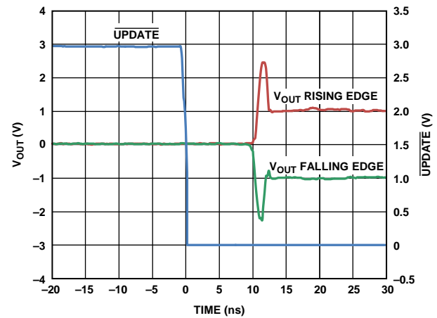
Figure 47. ADV3225 Enable Time
