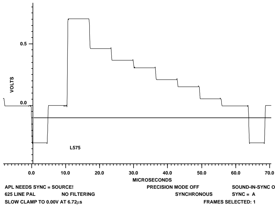
Figure 84. 100/0/75/0 PAL Color Bars Luminance
