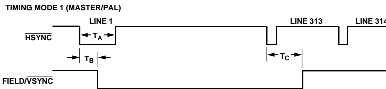
Figure 44. Timing Register 1
