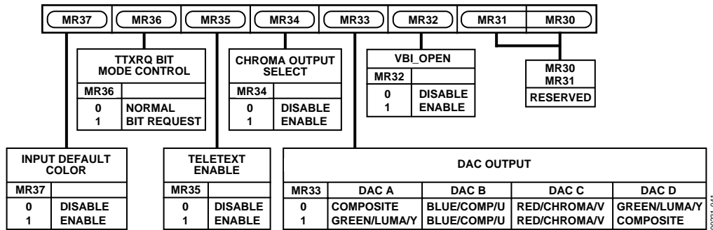
Figure 41. Mode Register 3
