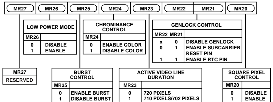
Figure 40. Mode Register 2
