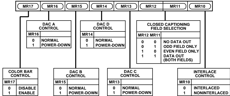
Figure 39. Mode Register 1
