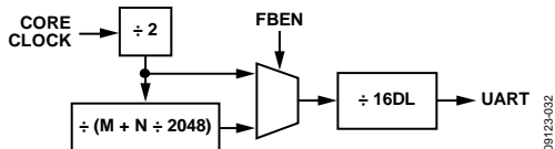
Figure 48. Baud Rate Generation Options
