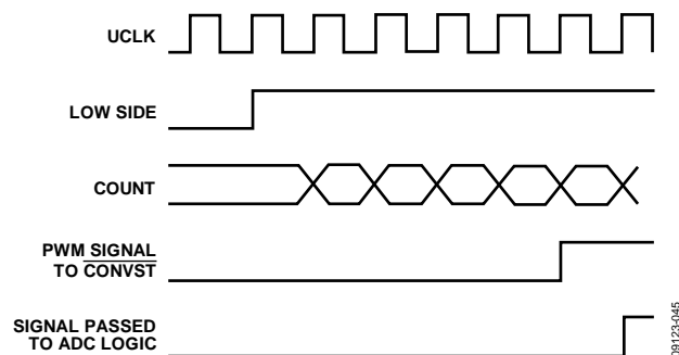
Figure 50. ADC Conversion
