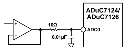
Figure 37. Buffering Single-Ended/Pseudo Differential Input
