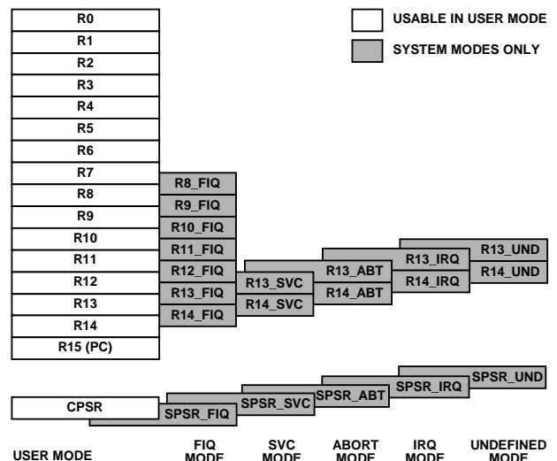
Figure 23. Register Organization
