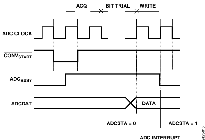
Figure 31. ADC Timing
