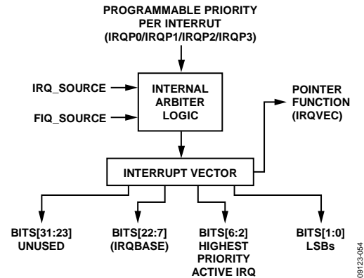
Figure 52. Interrupt Structure
