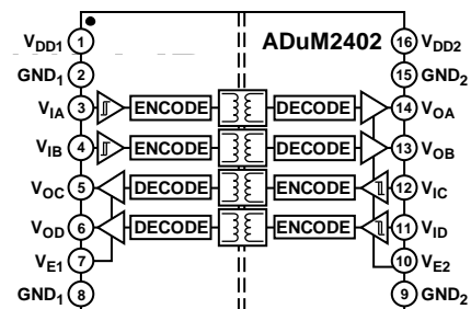
Figure 3. ADuM2402
