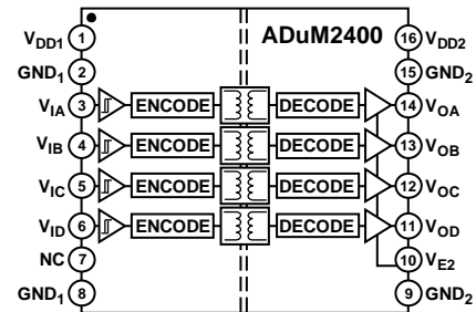
Figure 1. ADuM2400
