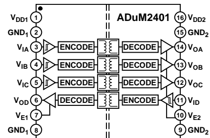
Figure 2. ADuM2401
