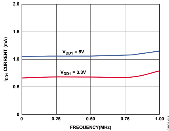
Figure 9. Typical I_{DD1} Supply Current vs. Frequency
