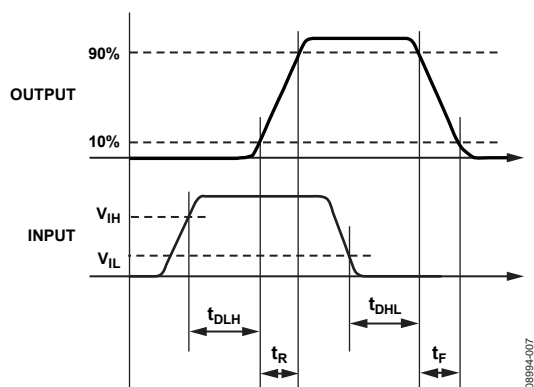
Figure 18. Propagation Delay Parameters
