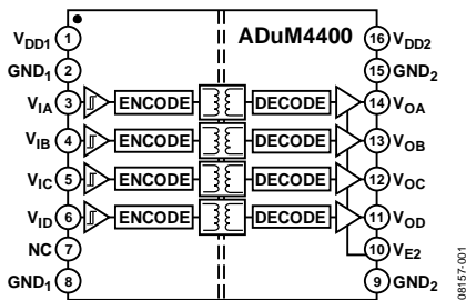
Figure 1. ADuM4400
