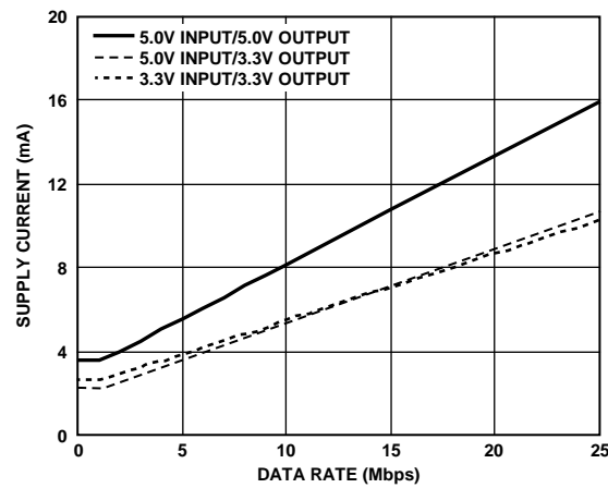
Figure 19. Typical I_{CHn} Supply Current per Forward Data Channel (15 pF Output Load)
