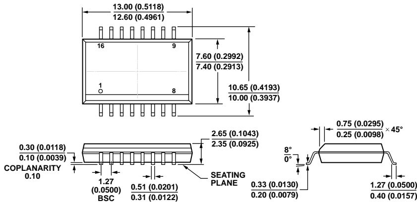
Figure 31. 16-Lead Standard Small Outline Package [SOIC_W] Wide Body (RW-16) Dimensions shown in millimeters and (inches)
