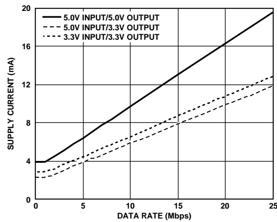
Figure 20. Typical I_{CHn} Supply Current per Reverse Data Channel (15 pF Output Load)
