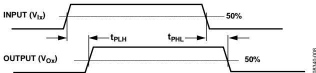
Figure 17. Propagation Delay Parameters
