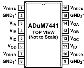
Figure 6. ADuM7441 Pin Configuration
