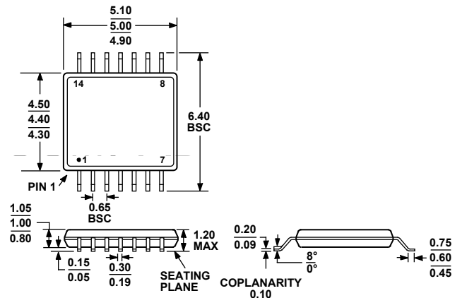
Figure 77. 14-Lead Thin Shrink Small Outline Package [TSSOP] (RU-14)
