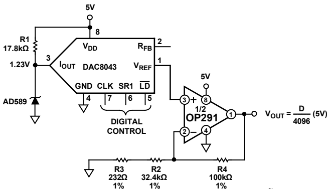
Figure 68. 5 V Only, 12-Bit DAC Swings Rail-to-Rail
