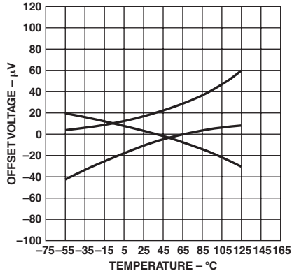
TPC 10. Offset Voltage Drift of Representative Units
