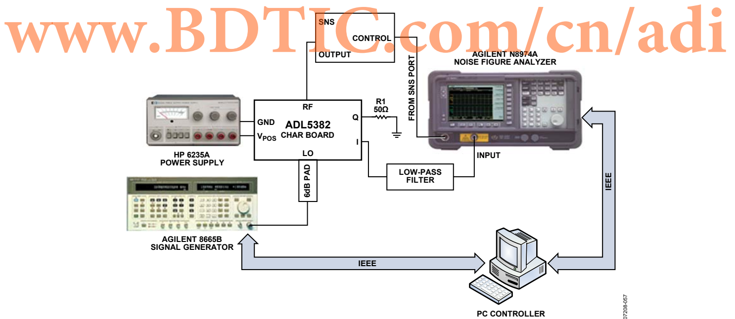
Figure 57. General Noise Figure Measurement Setup
