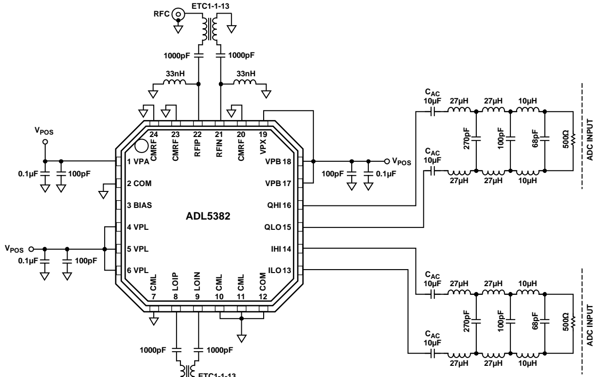
Figure 53. Sixth-Order Low-Pass Butterworth, Baseband Filter Schematic
