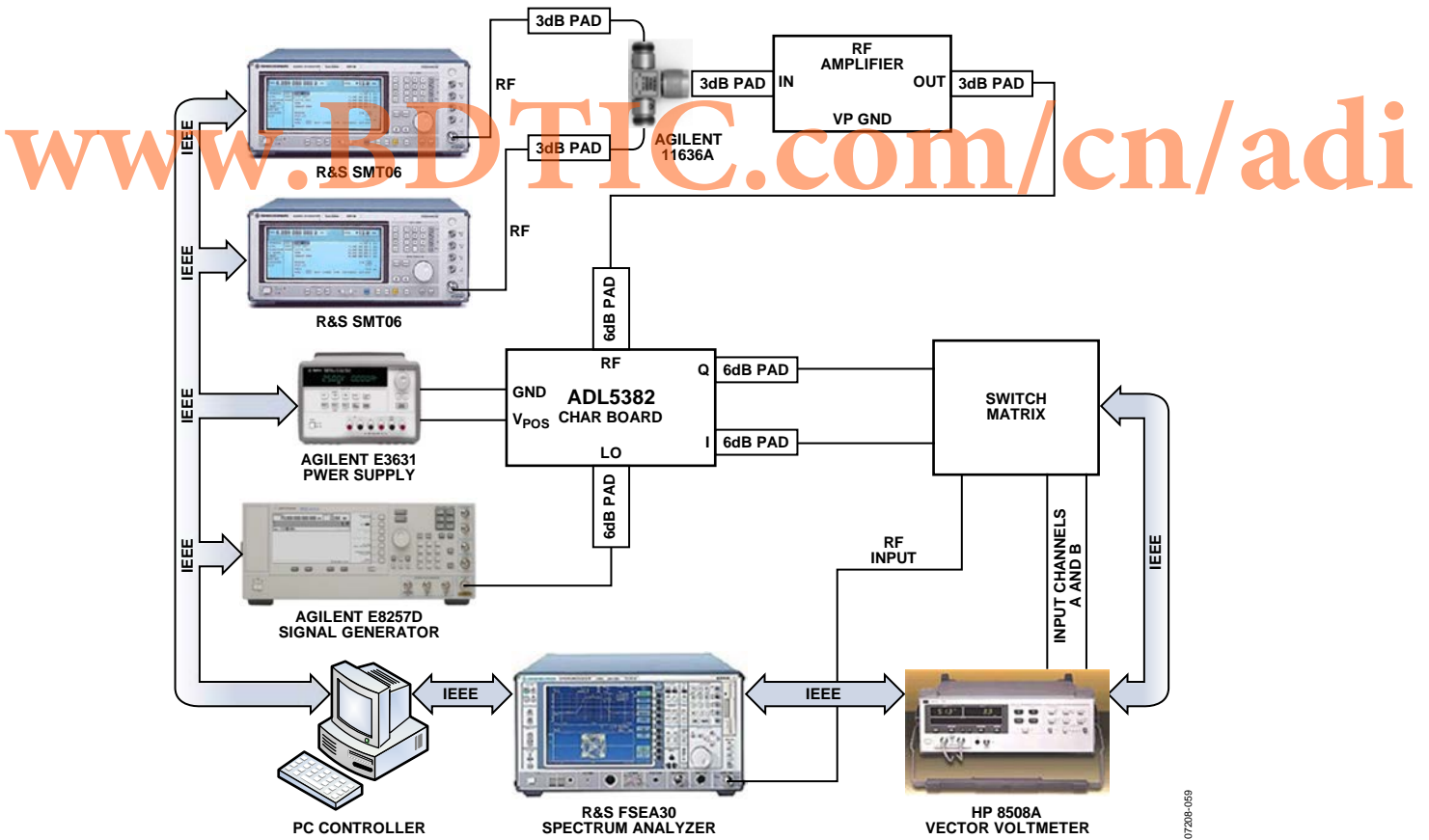
Figure 59. General Characterization Setup
