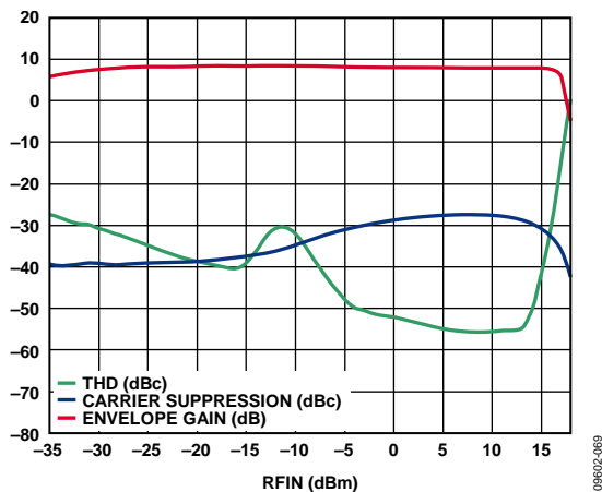
Figure 51. THD on V_{ENV} vs. RF Input Level; 1900 MHz RF Input, AM Modulated by a 20 MHz Sine Wave (Modulation Index = 0.25), V_{ENV} Output AC-Coupled into a 50 Ω Spectrum Analyzer Load
