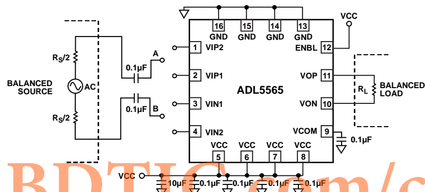
Figure 31. Basic Connections
