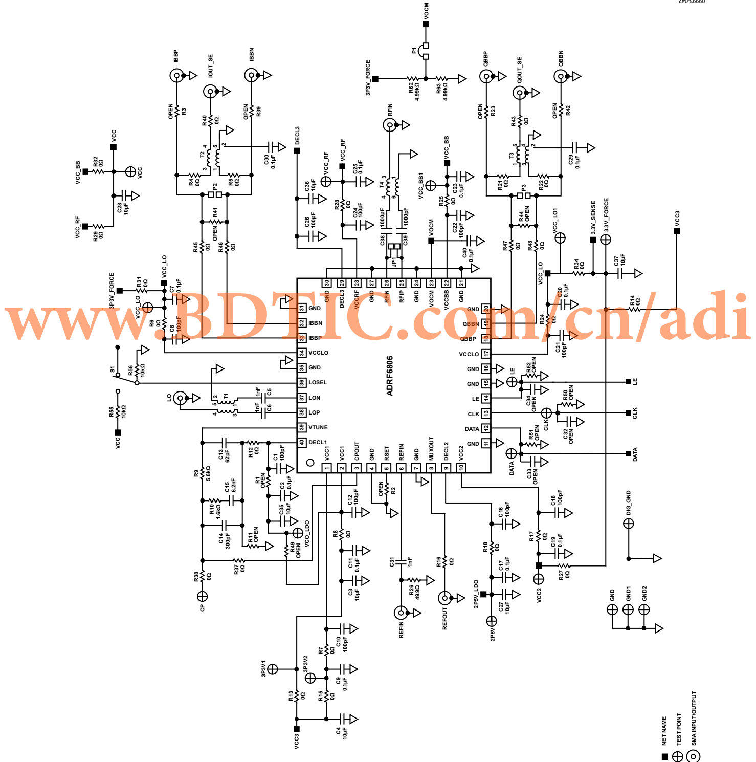
Figure 43. Evaluation Board Schematic
