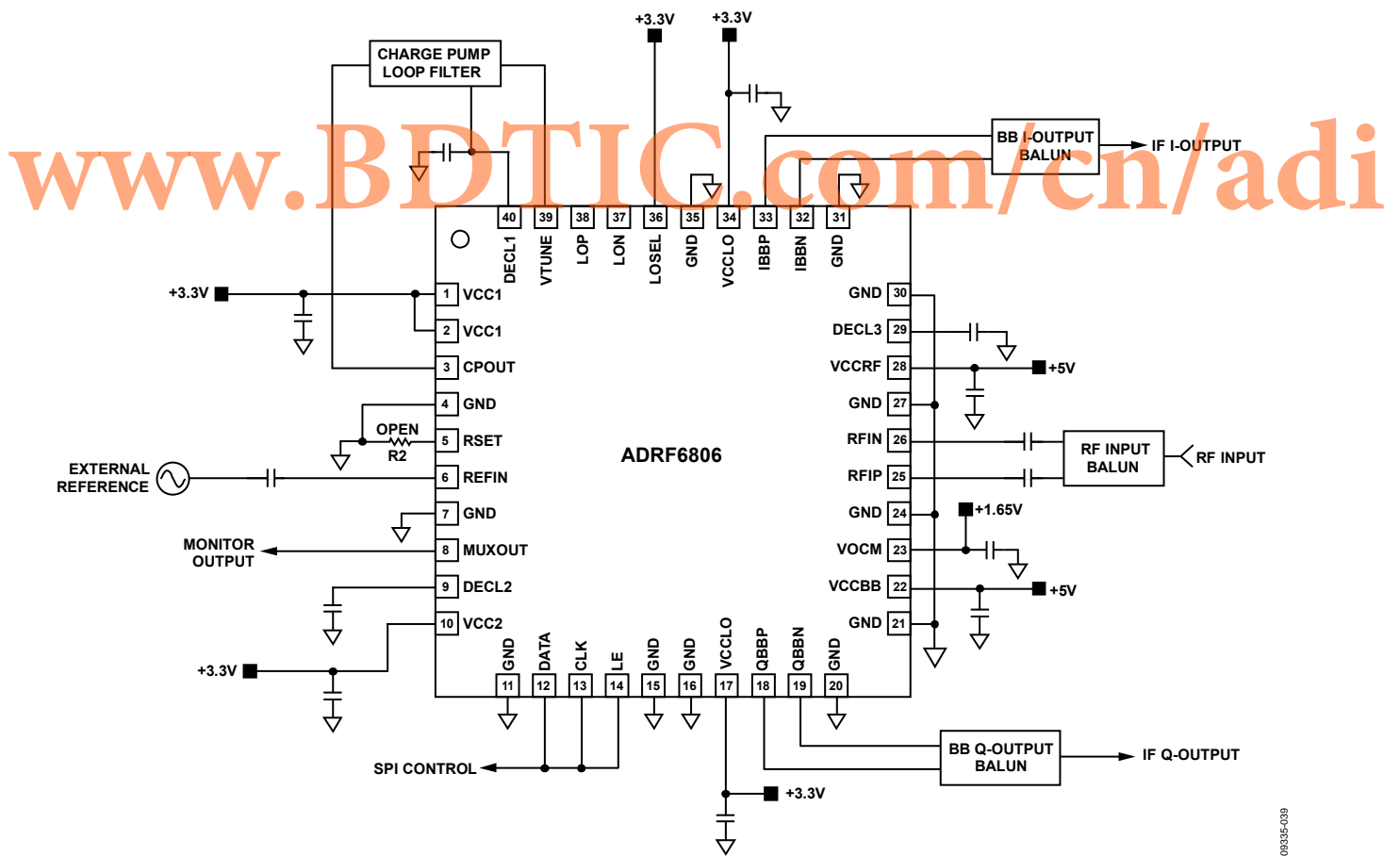
Figure 41. Basic Connections
