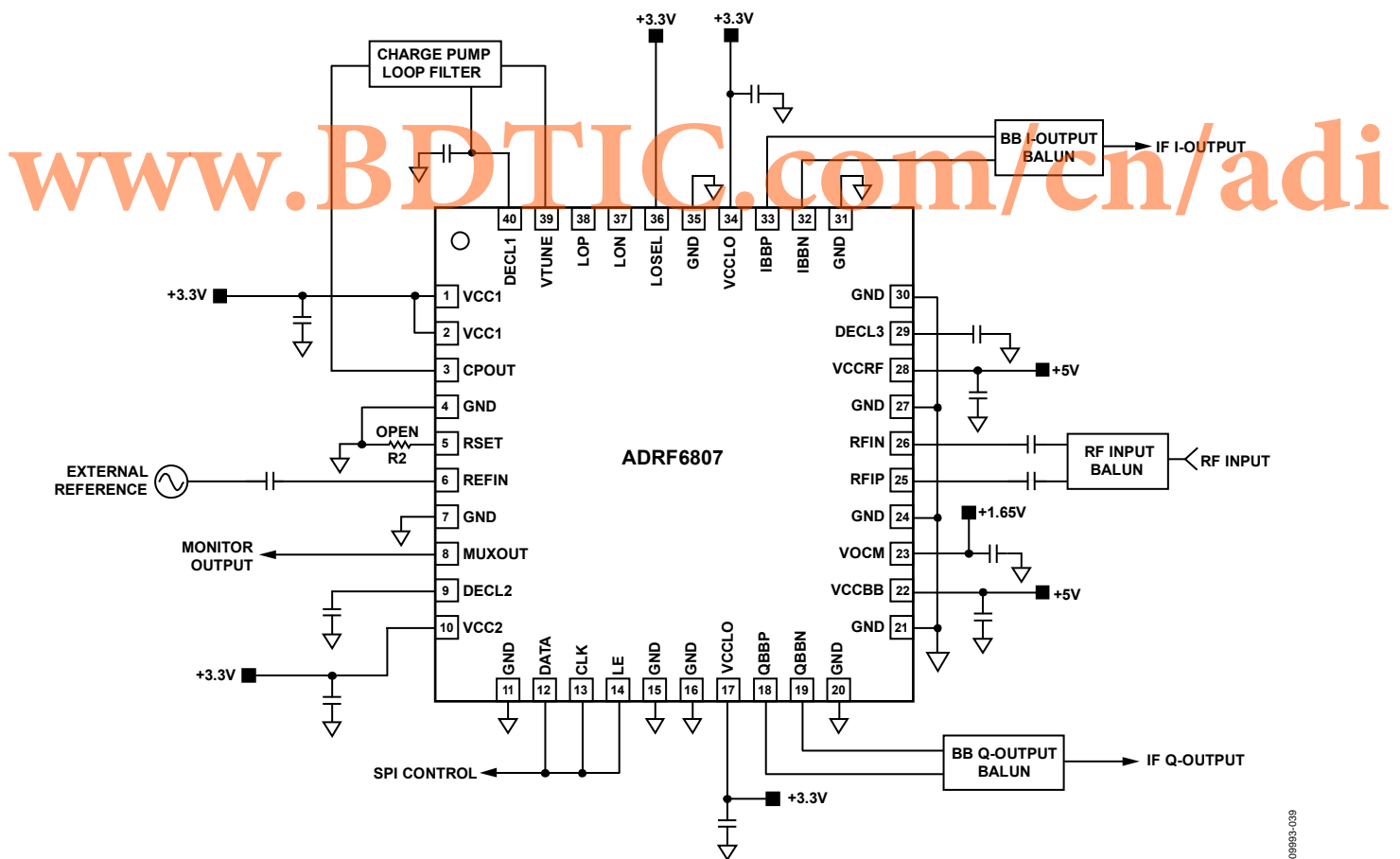
Figure 41. Basic Connections
