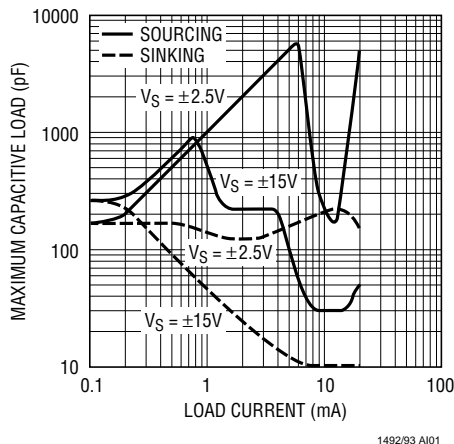
Maximum Capacitive Load vs Load Current
