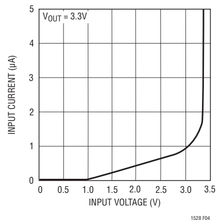
Figure 4. Input Current
