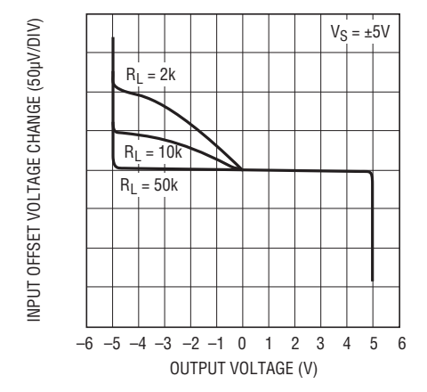
Open-Loop Gain
