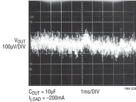
LT1964-5, 10Hz to 100kHz Output Noise, C_{BYP} = 1000pF
