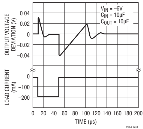
LT1964-5, Transient Response, C_{BYP} = 0.01\mu F
