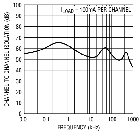
Channel-to-Channel Isolation
