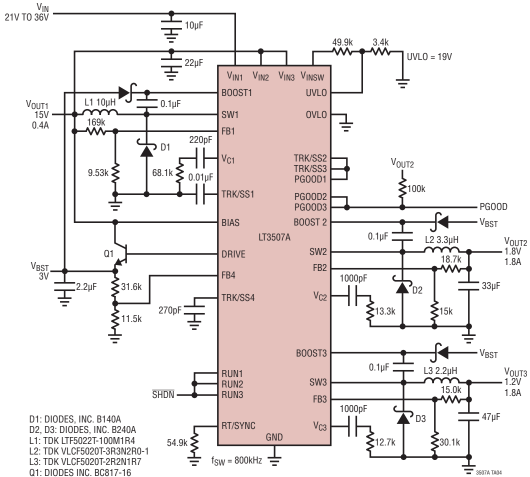
15V, 1.8V and 1.2V 2-Stage Step Down
