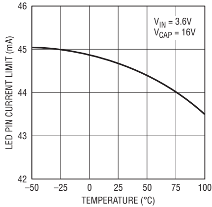
LED Pin Current Limit
