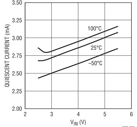
Quiescent Current ( V_{CTRL} = 3.6\text{V} )
