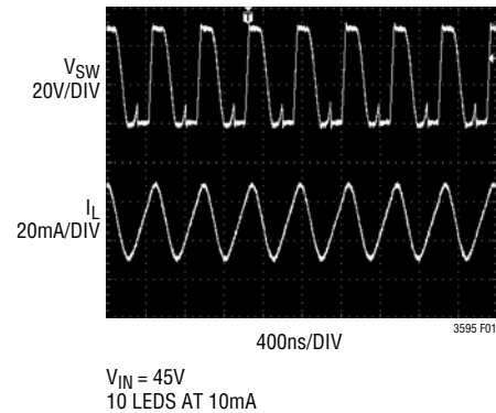
Figure 1. Switching Waveforms
