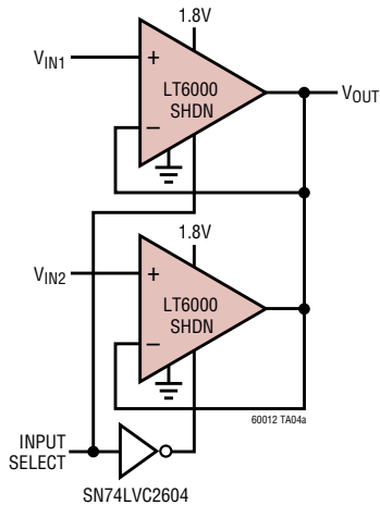
MUX Amplifier
