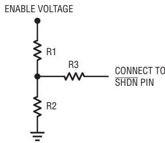
Figure 2. Programming Enable Voltage by Using External Resistors
