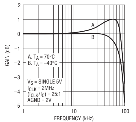
Maximum Passband vs Temperature
