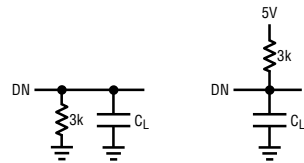
(A) V_{\text{OH}} TO Hi-Z
