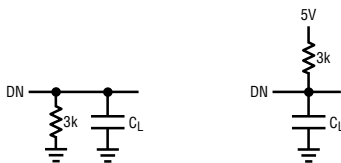
(A) Hi-Z TO V_{\text{OH}} AND V_{\text{OL}} TO V_{\text{OH}}
