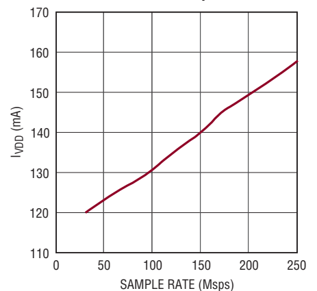
LTC2152-12: I_{OVD D} vs Sample Rate, 15MHz Sine Wave Input, -1\text{dBFS}
