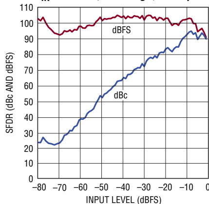
LTC2171-12: SFDR vs Input Level, f_{IN} = 70\text{MHz} , 2\text{V} Range, 40\text{Mps}
